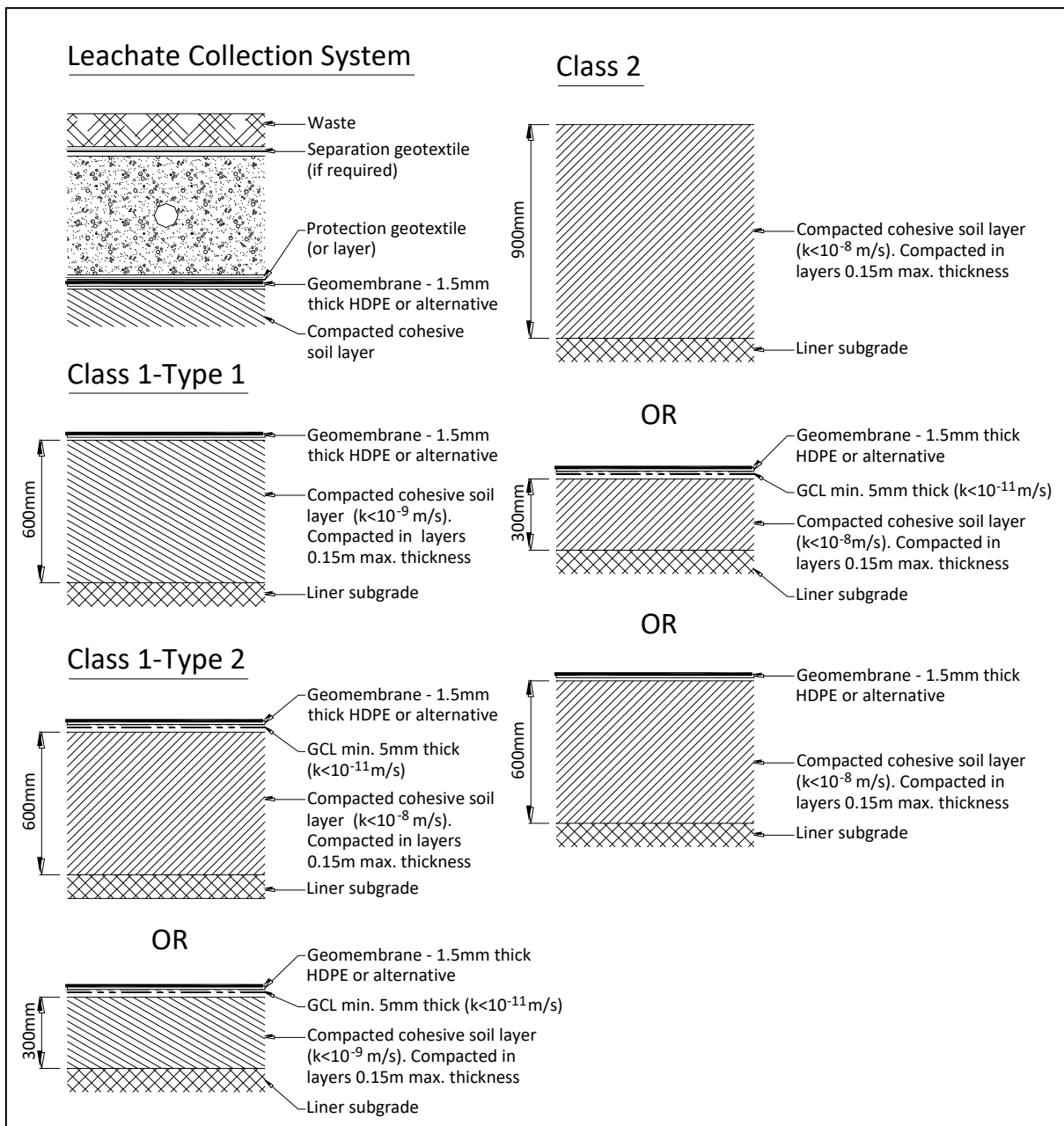
Figure 5-2 Liner Types
