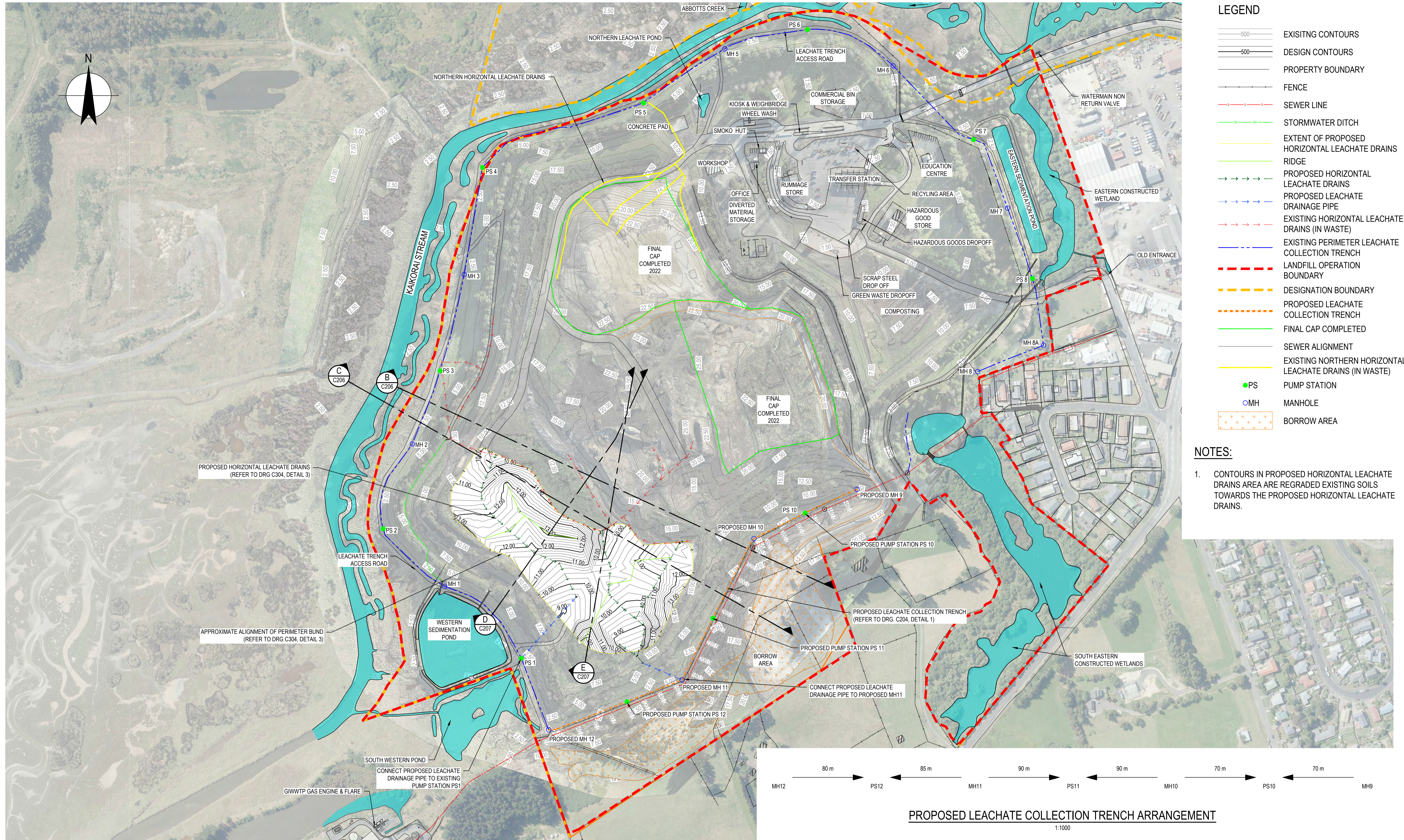
EXISTING AND PROPOSED LEACHATE COLLECTION SYSTEM - GENERAL ARRANGEMENT SCALE 1:1000
