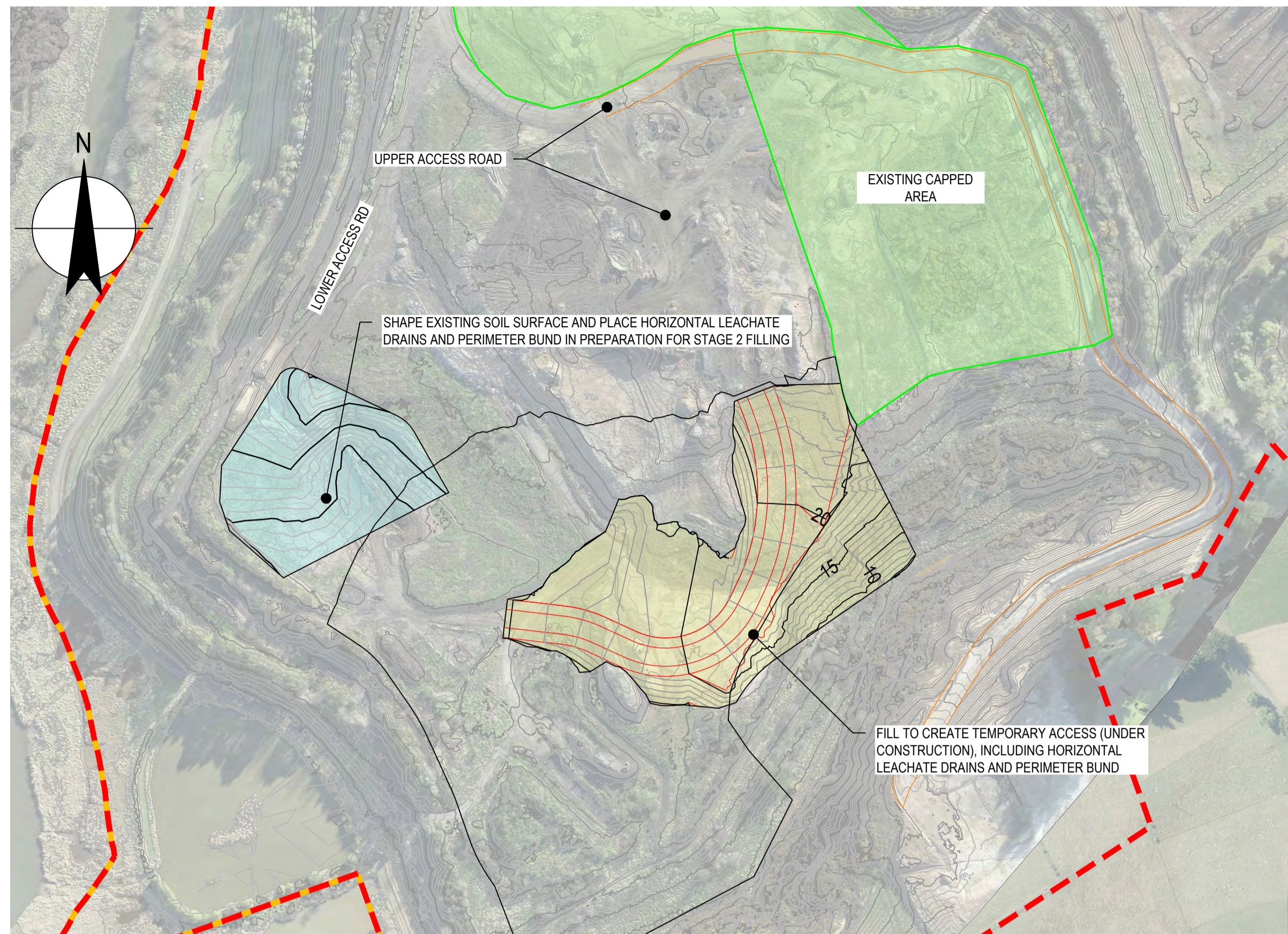
STAGE 1 WORKS SCALE 1:2000
