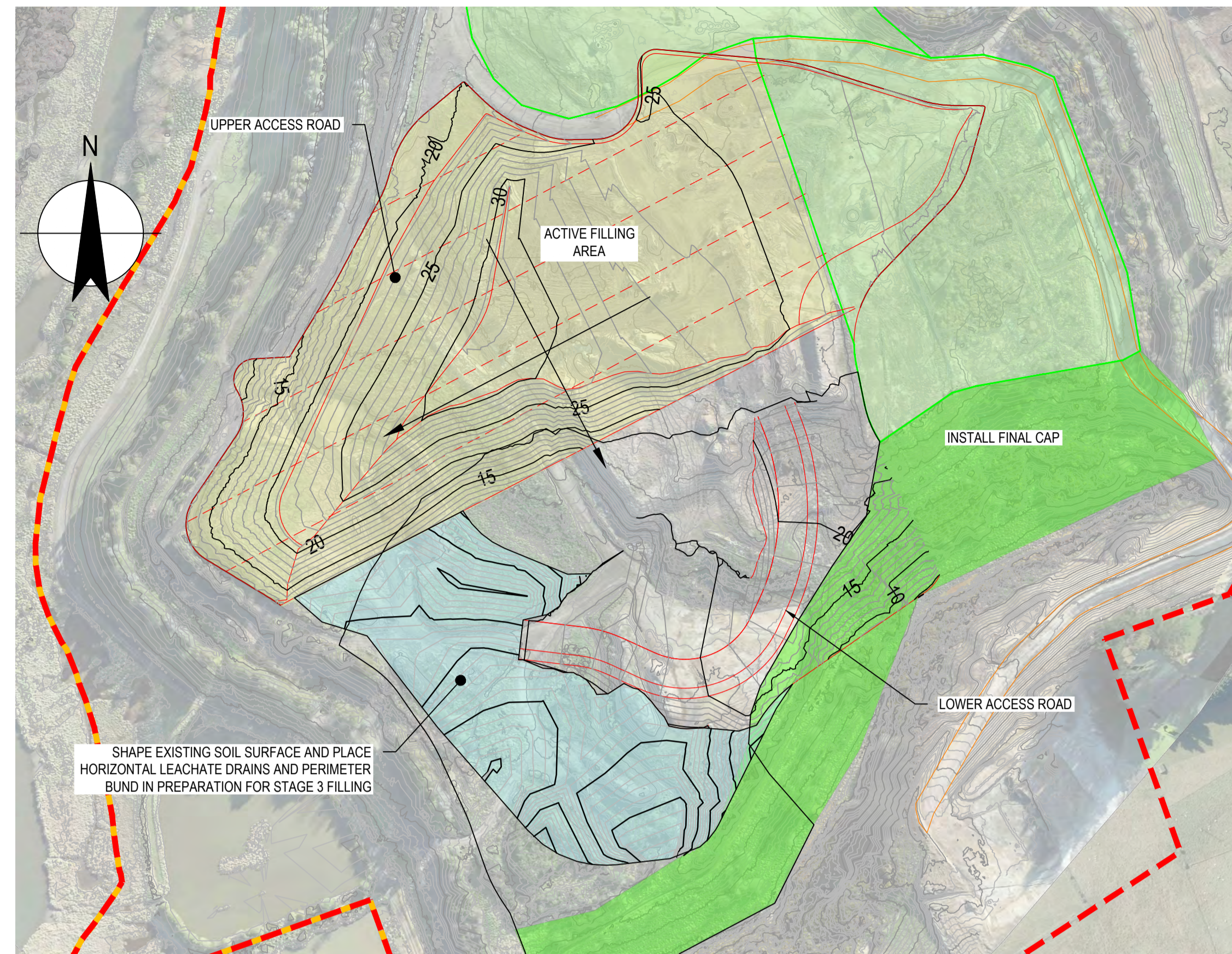
STAGE 2 WORKS SCALE 1:2000
