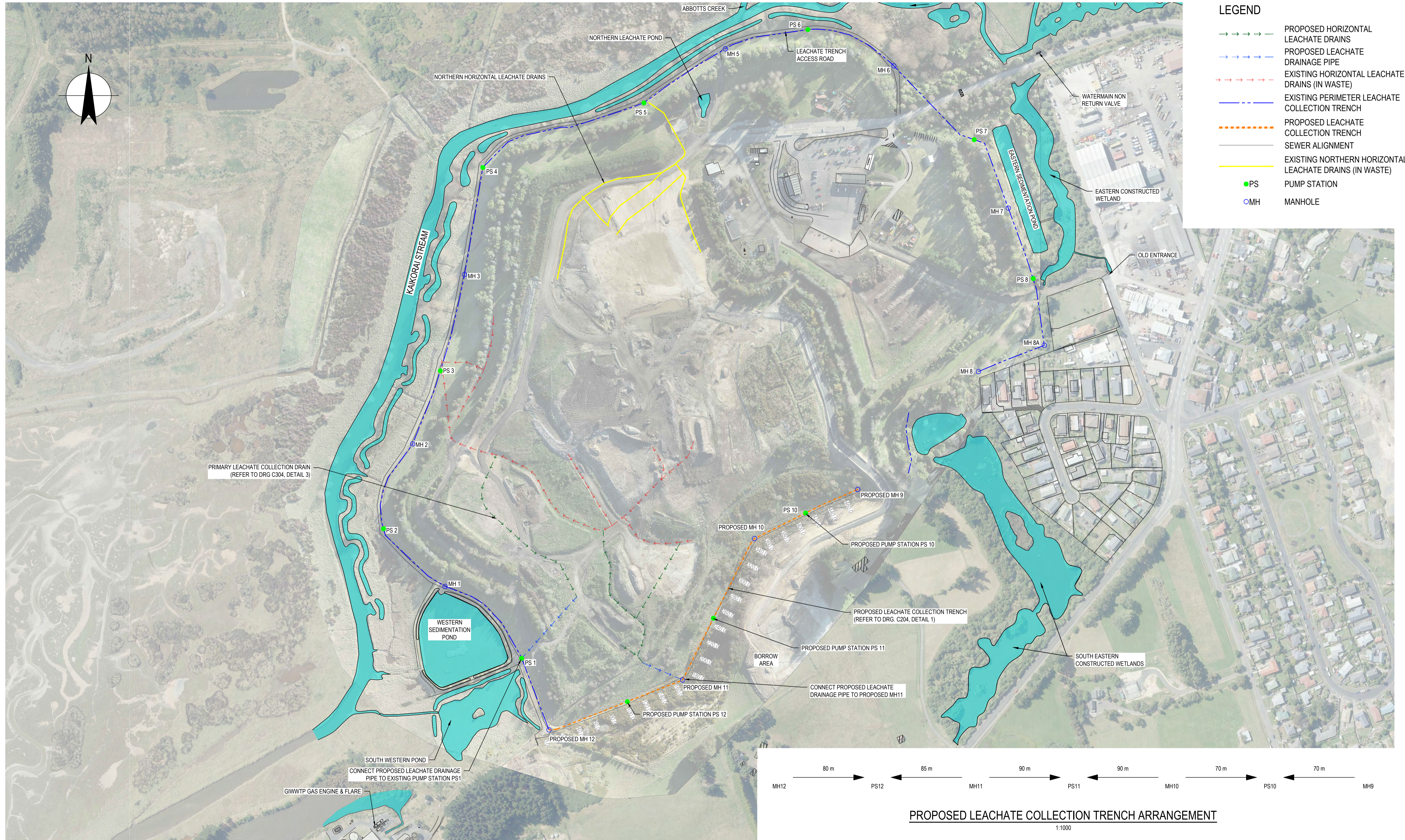
LAYOUT OF EXISTING AND PROPOSED LEACHATE COLLECTION SYSTEM ONLY SCALE 1:1000
