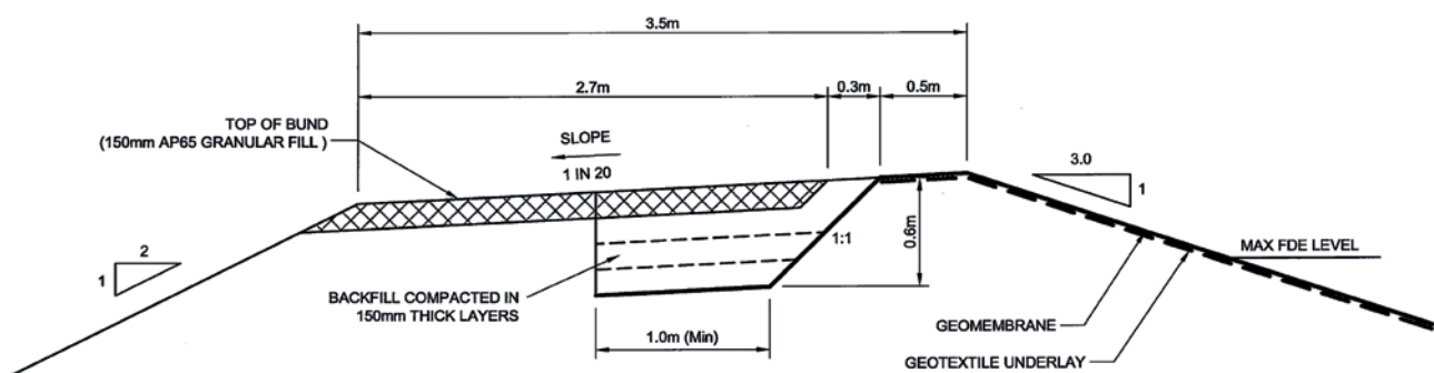
TYPICAL POND LINER ANCHOR DETAIL
