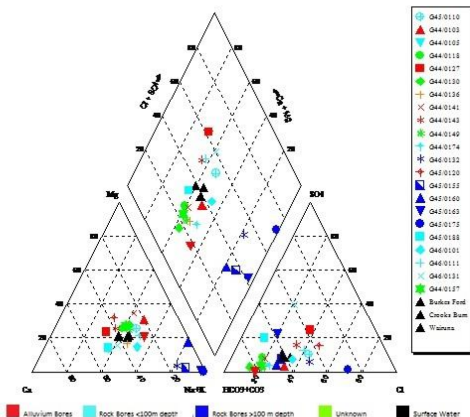
Figure 11 Tri-linear piper diagram – South Otago bores
