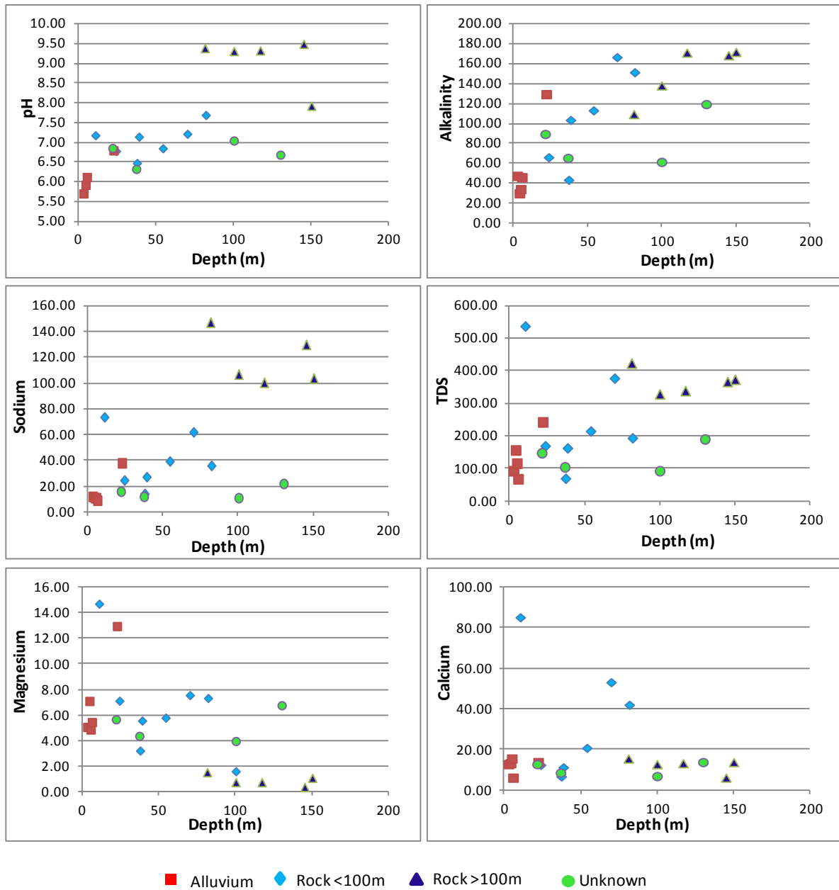
Figure 13 Trends in chemistry in groundwater basins in South Otago (continued)
