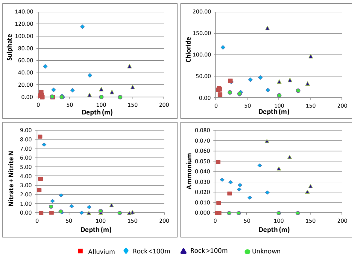
Figure 12 Trends in chemistry in groundwater in South Otago
