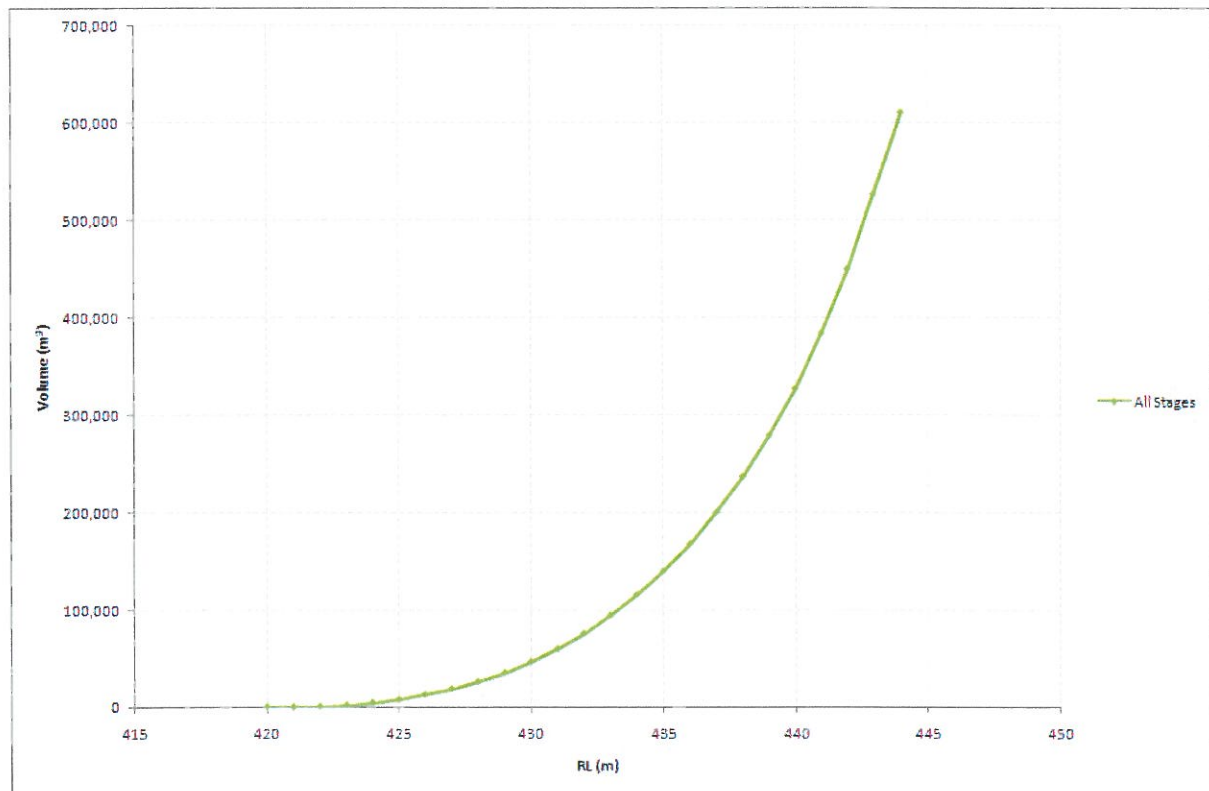
Figure 6: Lone Pine Reservoir volume to RL assumptions (RL's in m).
