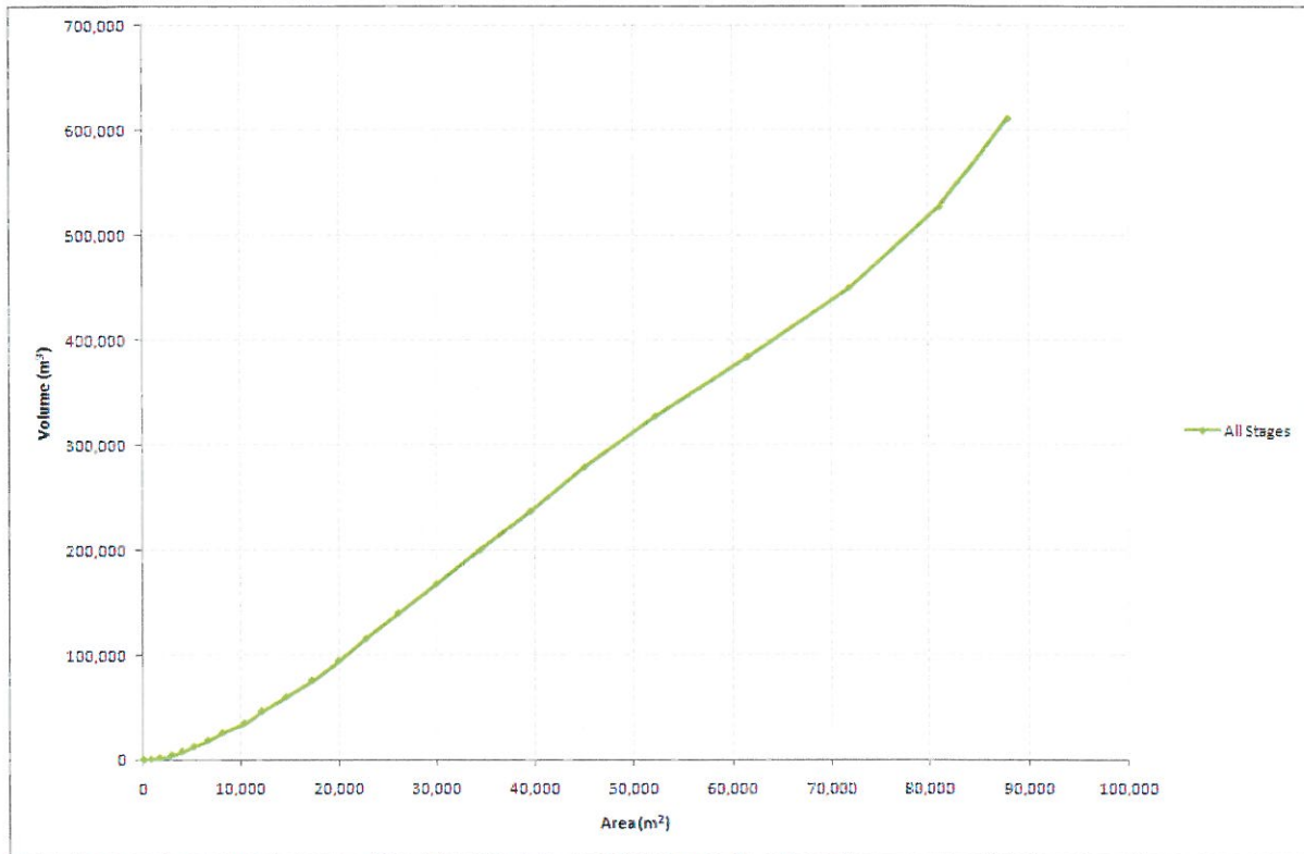
Figure 5: Lone Pine Reservoir volume to area assumptions (all areas in m 2 )
