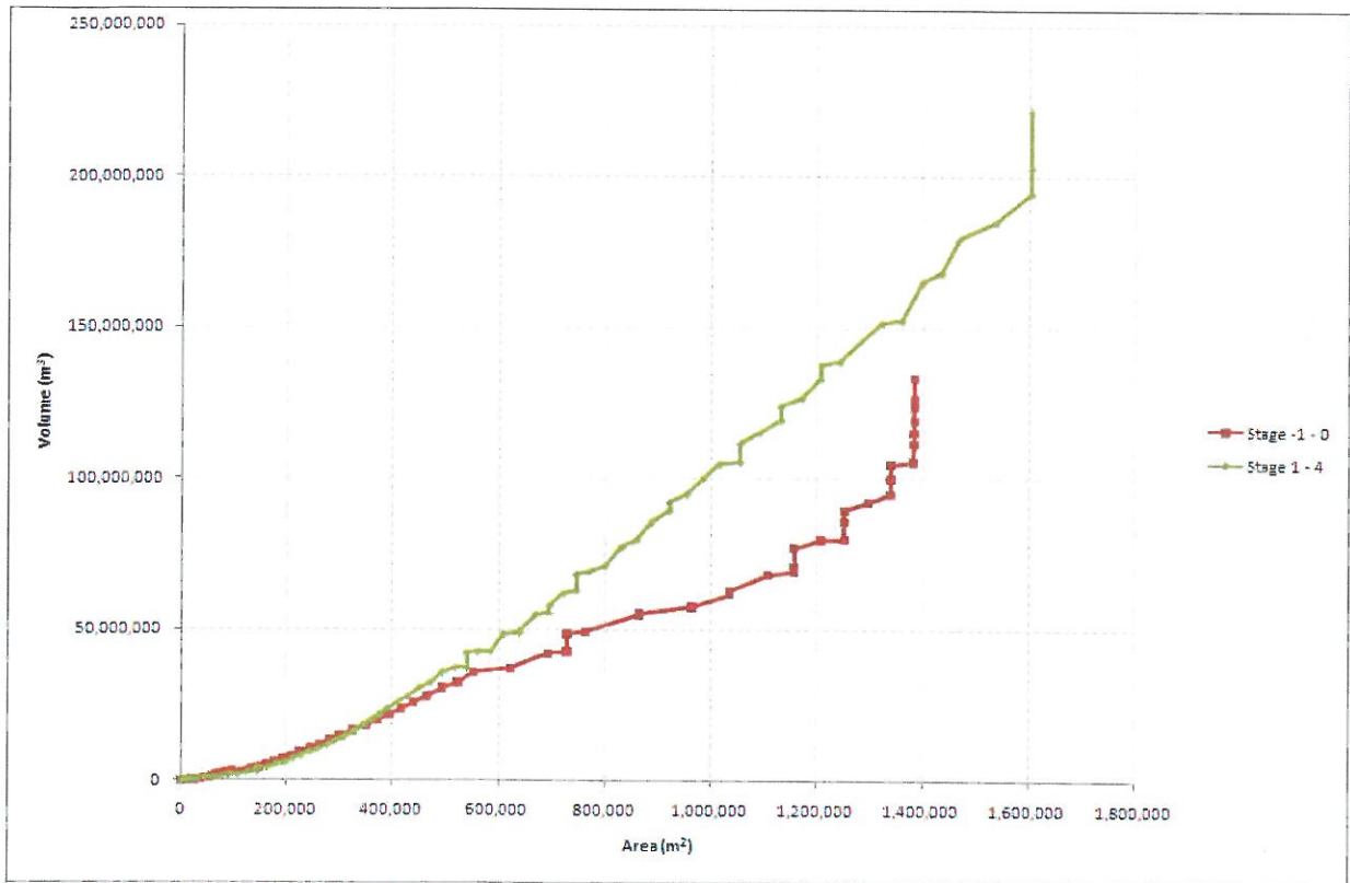
Figure 3: Frasers/Innes Mills Pit volume to area assumptions (all areas in m2)
