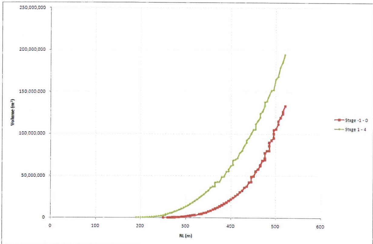
Figure 4: Frasers/Innes Mills Pit volume to RL assumptions (RL's in m).
