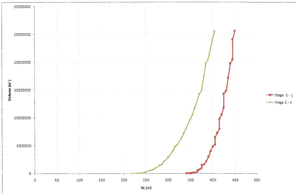
Figure 2: Roundhill/Golden Point/Southern Pit volume to RL assumptions (RL's in m).
