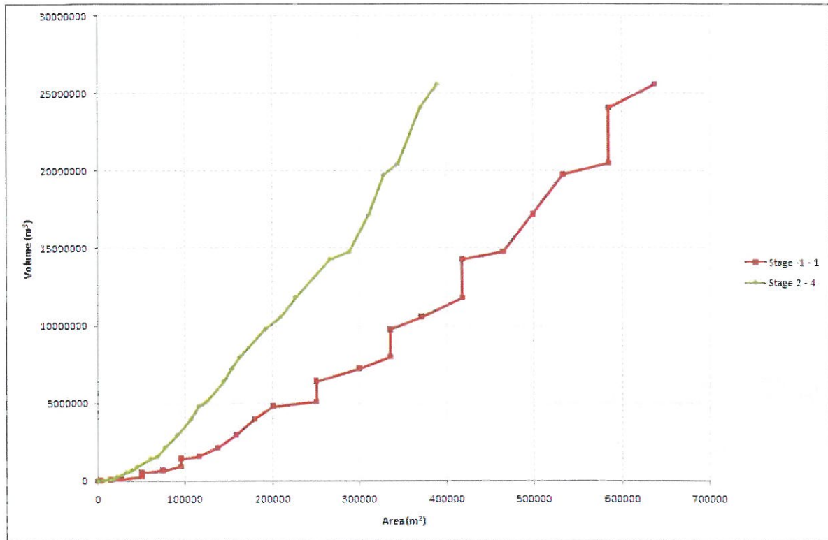
Figure 1: Roundhill/Golden Point/Southern Pit volume to area assumptions (all areas in m 2 ).
