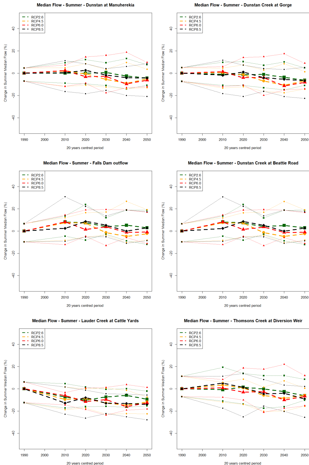
Figure G-7: 20-years centred change in Summer median flow characteristic across RCPs over the period 2006-2060 at six locations in the Manuherekia catchment. Top left plot shows the changes for Dunstan at Manuherekia, the top right plot shows the changes for Dunstan Creek at Gorge, the middle left plot shows the changes for Falls Dam outflow, middle right plot shows the changes for Dunstan Creek at Beattie Road, bottom left plot shows the change for Lauder Creek at Cattle Yards and bottom right shows the changes for Thomsons Creek at Diversion Weir.
