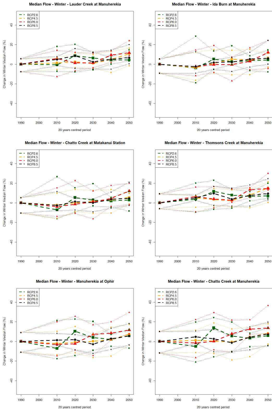
Figure G-11: 20-years centred change in Winter median flow characteristic across RCPs over the period 2006-2060 at six locations in the Manuherekia catchment. Top left plot shows the changes for Lauder Creek at Manuherekia, the top right plot shows the changes for Ida Burn at Manuherekia, the middle left plot shows the changes for Chatto Creek at Matakanui Station, middle right plot shows the changes for Thomsons Creek at Manuherekia, bottom left plot shows the change for Manuherekia at Ophir and bottom right shows the changes Chatto Creek at Manuherekia.
