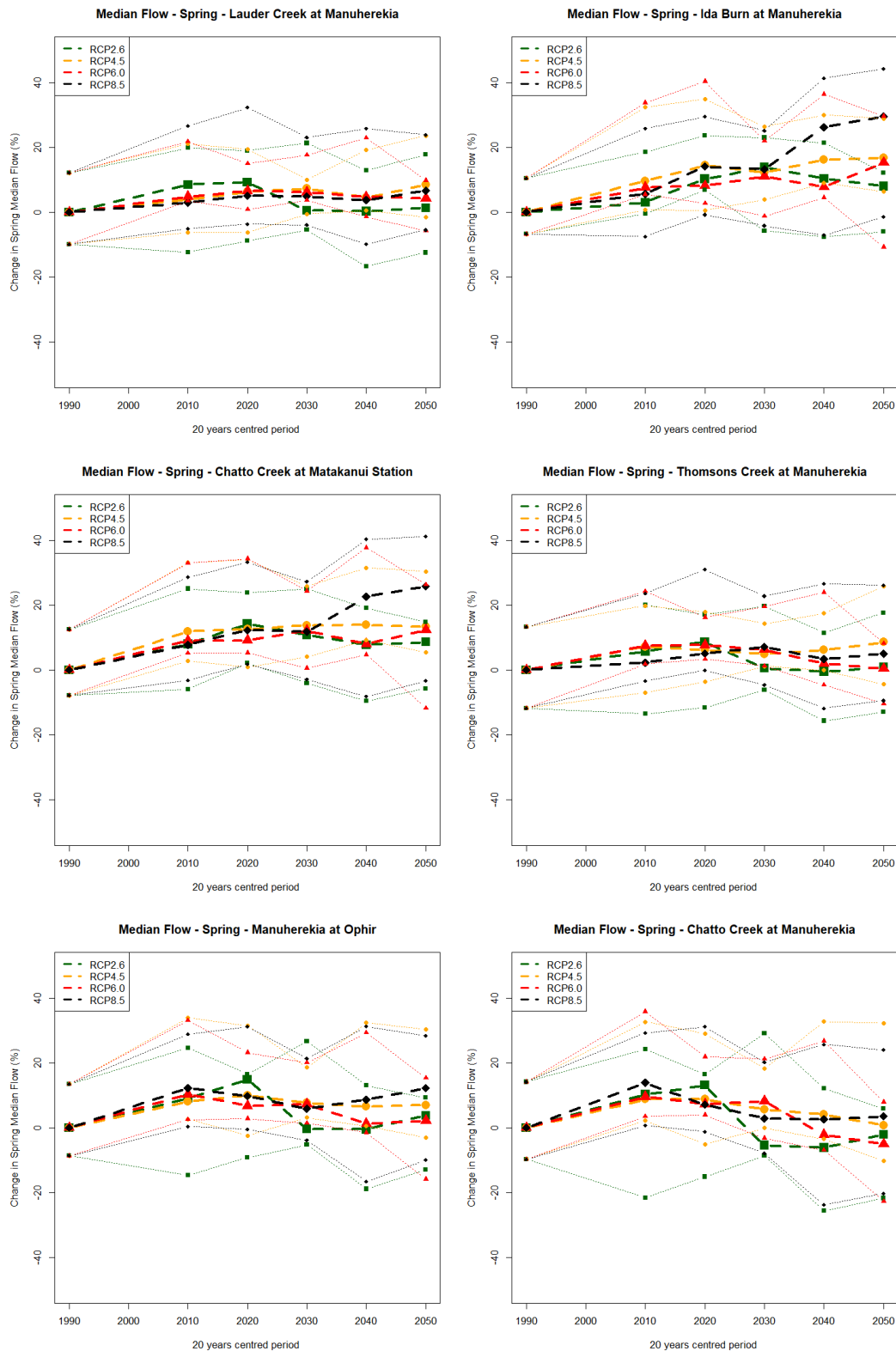
Figure G-5: 20-years centred change in Spring median flow characteristic across RCPs over the period 2006-2060 at six locations in the Manuherekia catchment. Top left plot shows the changes for Lauder Creek at Manuherekia, the top right plot shows the changes for Ida Burn at Manuherekia, the middle left plot shows the changes for Chatto Creek at Matakanui Station, middle right plot shows the changes for Thomsons Creek at Manuherekia, bottom left plot shows the change for Manuherekia at Ophir and bottom right shows the changes Chatto Creek at Manuherekia.
