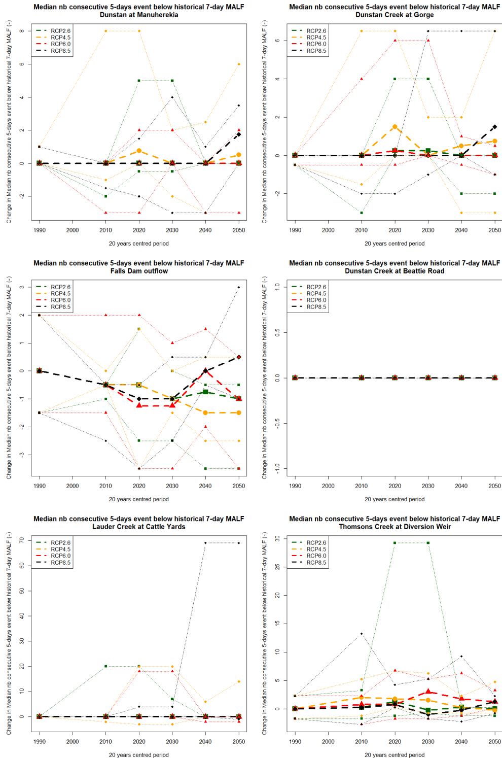
Figure J-4: 20-years centred change in median number of consecutive five day events below historical 7-day MALT across RCPs over the period 2006-2060 at six locations in the Manuhereikia catchment. Top left plot shows the changes for Dunstan at Manuherekia, the top right plot shows the changes for Dunstan Creek at Gorge, the middle left plot shows the changes for Falls Dam outflow, middle right plot shows the changes for Dunstan Creek at Beattie Road, bottom left plot shows the change for Lauder Creek at Cattle Yards and bottom right shows the changes for Thomsons Creek at Diversion Weir.
